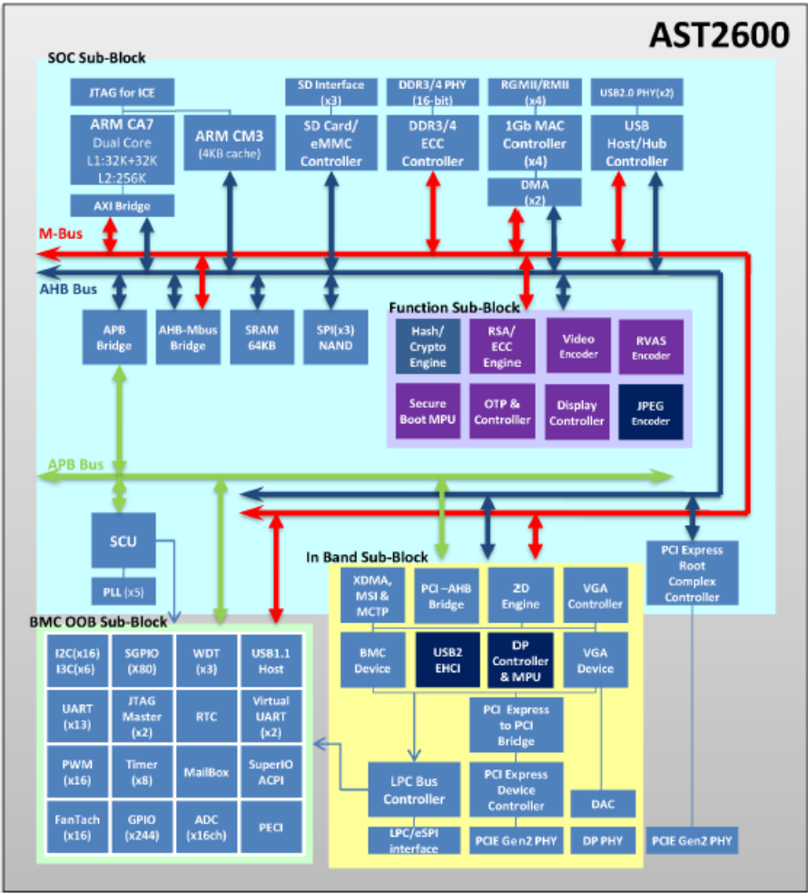
Figure A-1 AST2600 Chip Architecture
